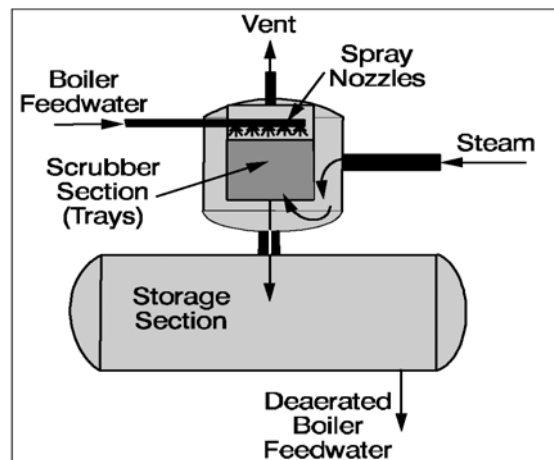
Figure 2.9 Deaerator
