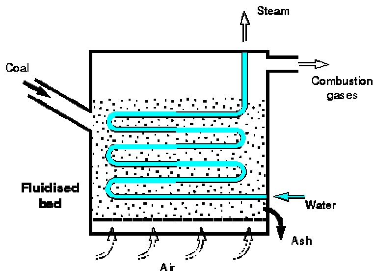
Figure 2.7 Fluidised Bed Combustion
