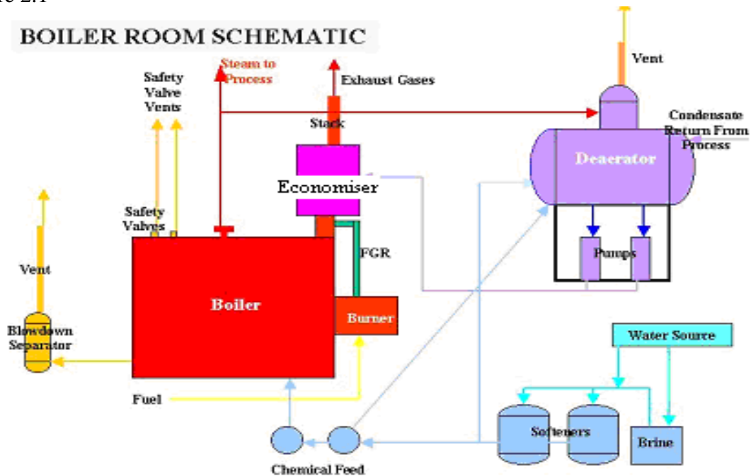
Figure 2.1 Boiler Room Schematic
