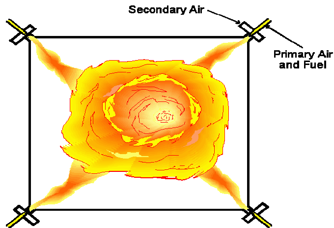
Figure 2.6 Tangential Firing
