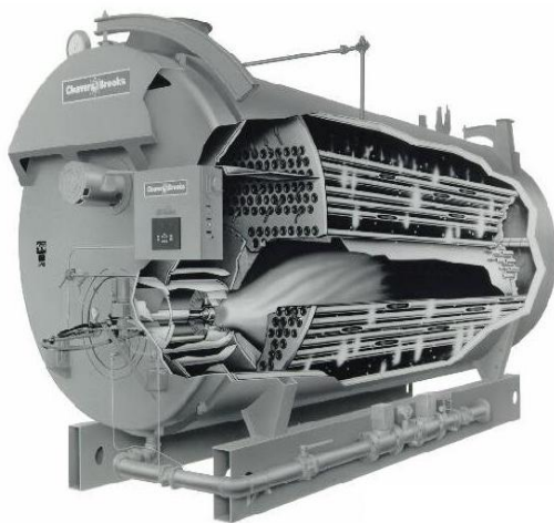
Figure 2.4 Packaged Boiler
