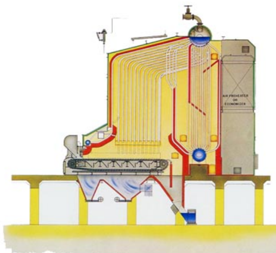
Figure 2.5 Chain Grate Stoker
