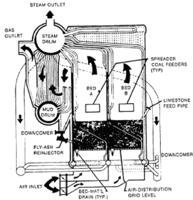
Figure 6.4 Bubbling Bed Boiler-2
