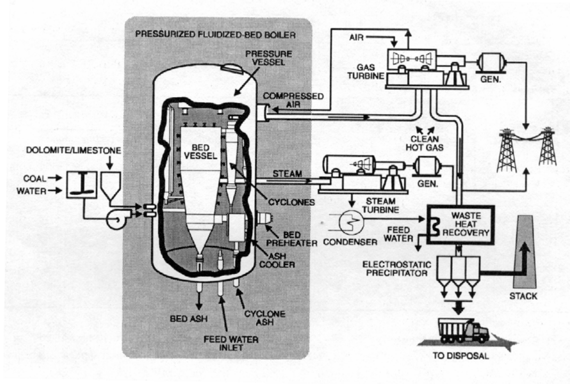
Figure 6.6 PFBC Boiler for Cogeneration
