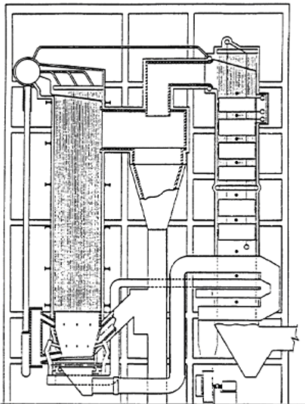
Figure 6.5 Circulating Bed Boiler Design
