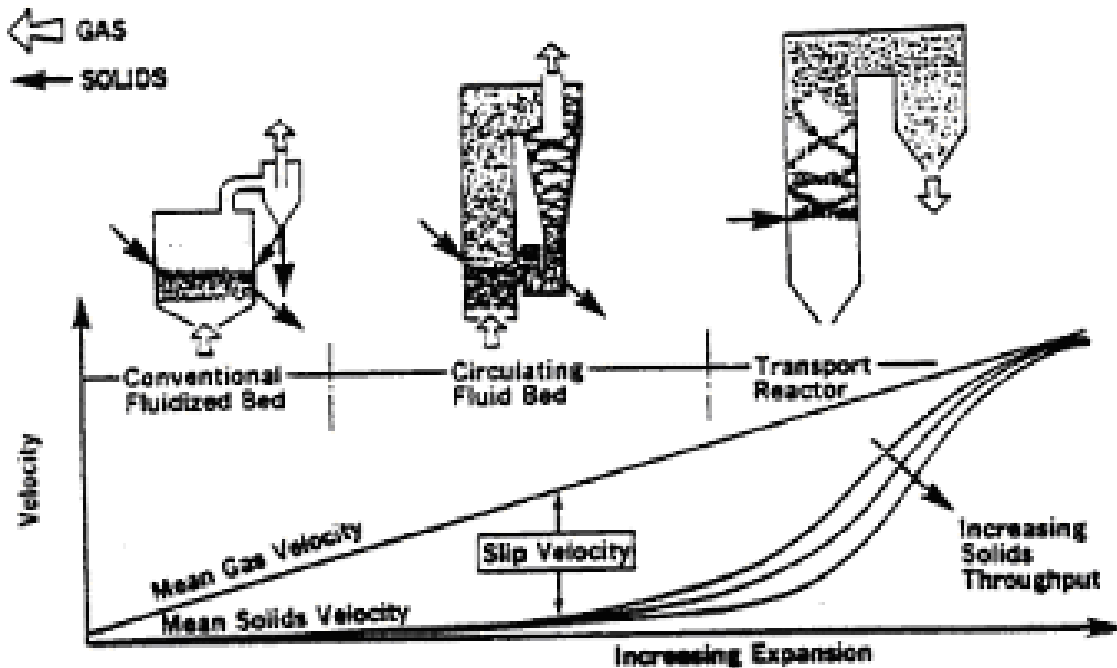
Figure 6.2 Relation between Gas Velocity and Solid Velocity
