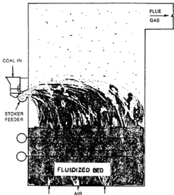
Figure 6.3 Bubbling Bed Boiler-1
