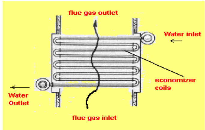
Figure 8.8 Economiser
