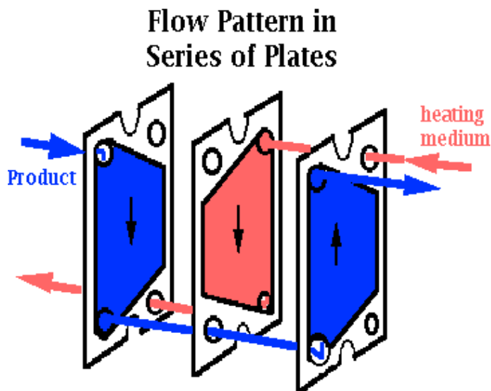
Figure 8.10 Plate Heat Exchanger
