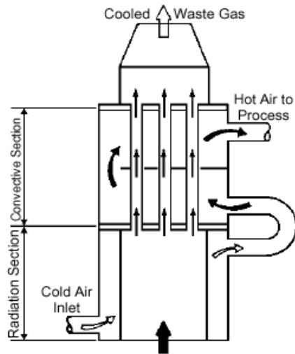
Figure 8.4 Convective Radiative Recuperator
