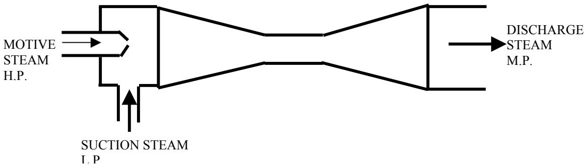
Figure 8.13 Thermocompressor
