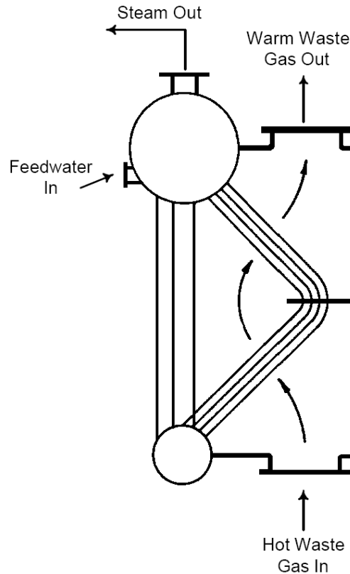
Figure 8.11 Two-Pass Water Tube Waste Heat Recovery Boiler
