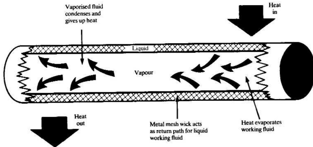
Figure 8.7 Heat Pipe
