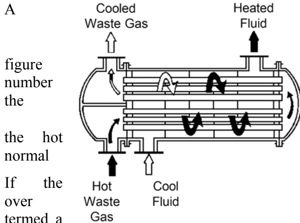
Figure 8.3 Convective Recuperator
