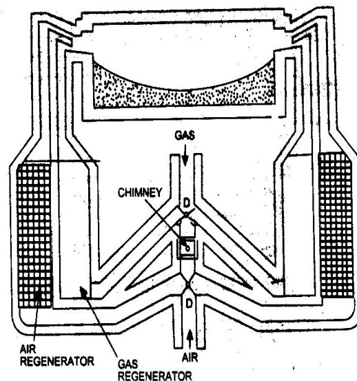
Figure 8.5 Regenerator
