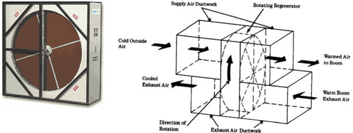
Figure 8.6 Heat Wheel
