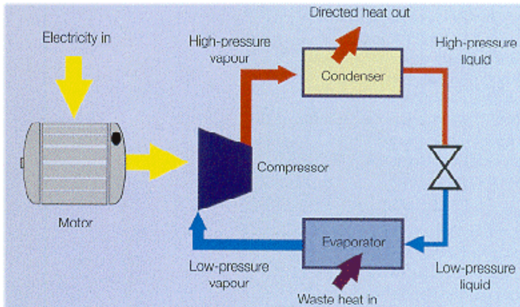
Figure 8.12 Heat pump
