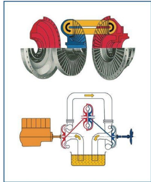
Figure 10.8 Fluid Coupling
