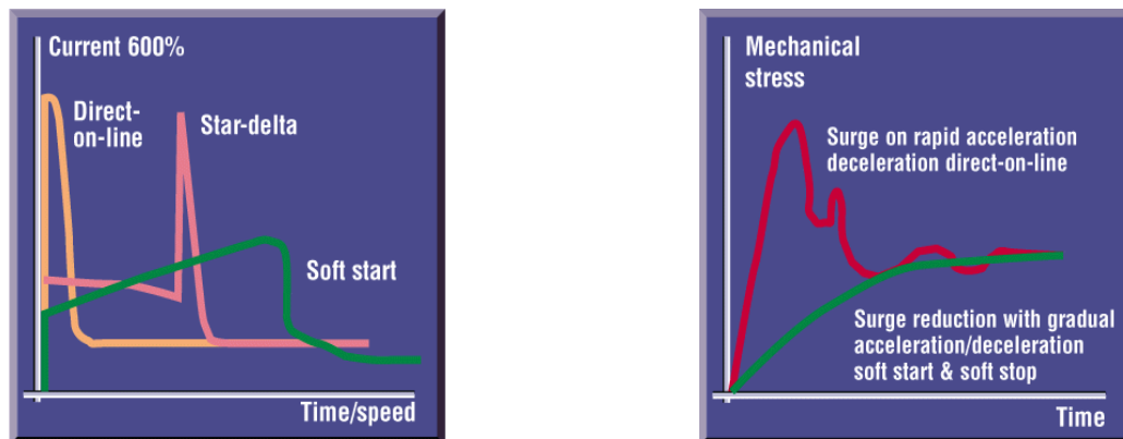
Figure 10.6 Soft Starter: Starting current, Stress profile during starting
