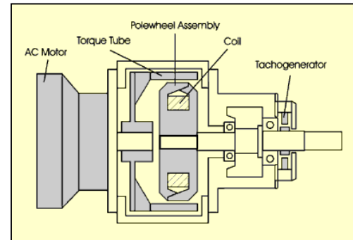
Figure 10.7 Eddy Current Drive
