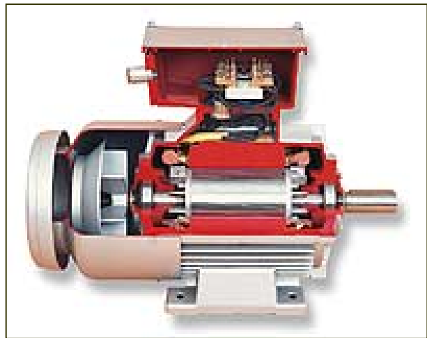
Figure 10.3 Energy Efficient Motor
