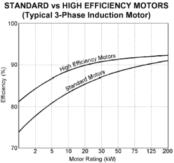
Figure 10.4 Efficiency Range for Standard and High Efficiency Motors
