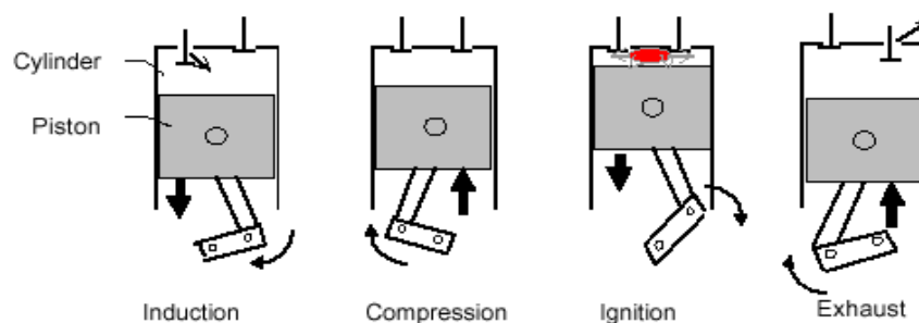
Figure –9.1 Schematic Diagram of Four-Stroke Diesel Engine
