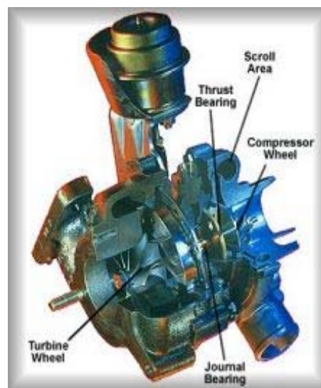
Figure – 9.3 Turbocharger
