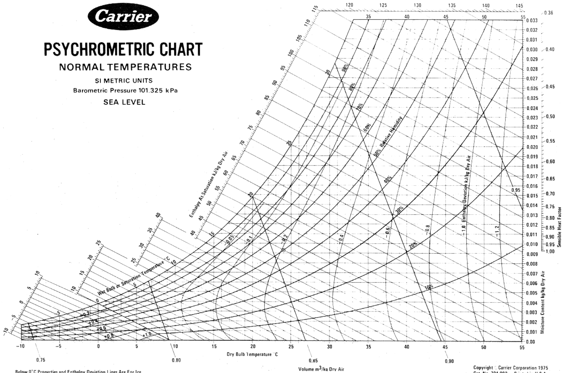
Figure 9.1 Psychrometric Chart
